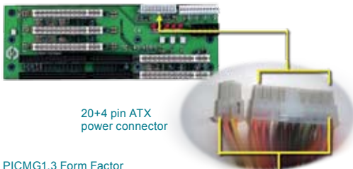
PICMG1.3 Form Factor Backplane PE-10S/6S
